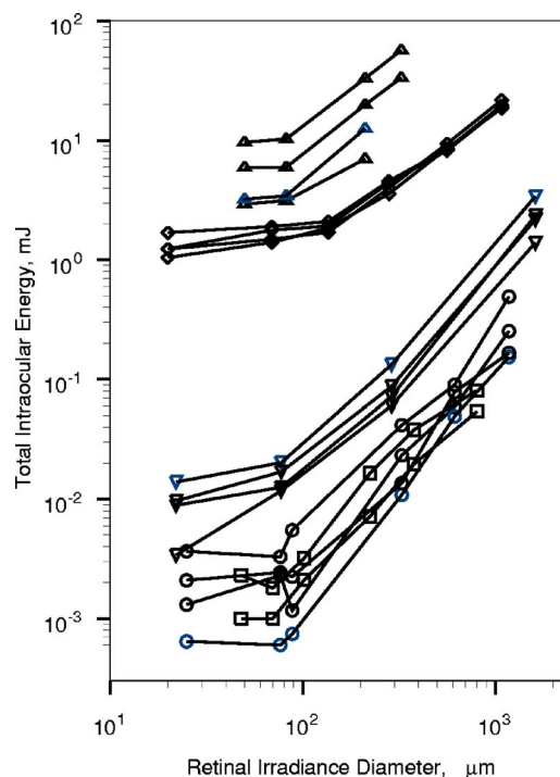
Fig. 5 Dependence of ED 50 on the retinal irradiance diameter for a range of exposure durations and laser wavelengths: squares, 150 fs and 1060 nm (Ref. 16); circles, 7 ns and 532 nm (Refs. 6 and 7); inverted triangles, 3 μs and 590 nm (Refs. 6 and 7); diamonds, 100 ms and 514 nm (this paper); triangles, 0.125 to 1 s and 633 nm (Ref. 9).
